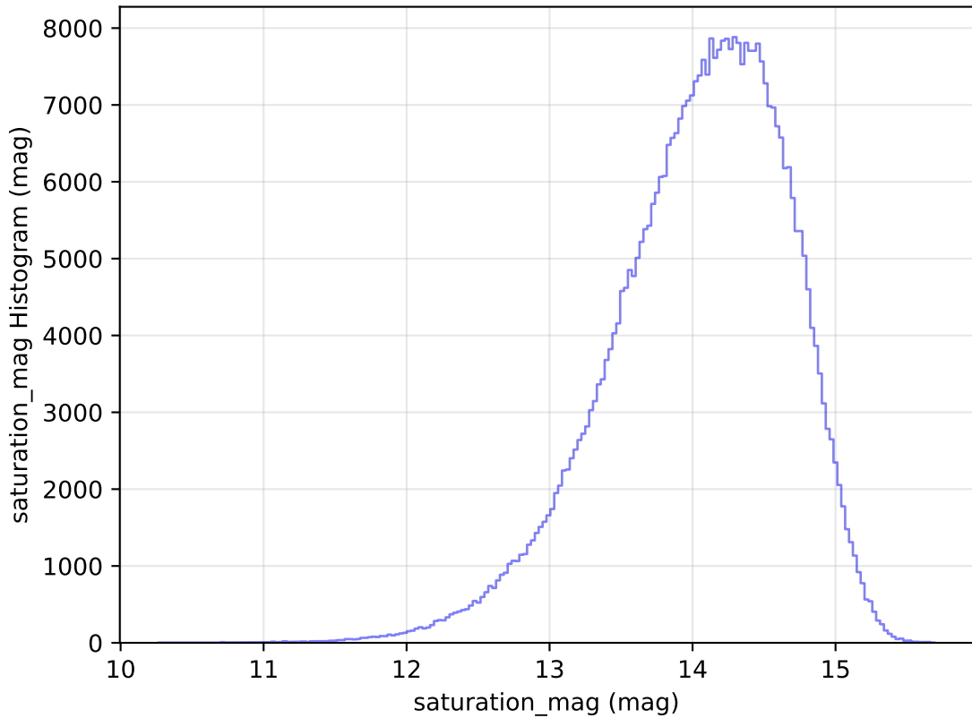
too_elab_heavy_r32_d2_gz_v3.4_10yrs All sky z band: saturation_mag Histogram
