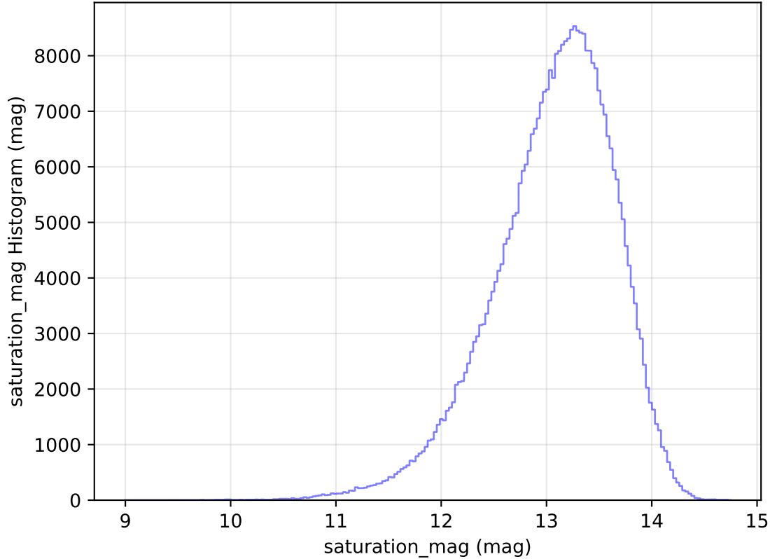
too_elab_heavy_r32_d2_gz_v3.4_10yrs All sky y band: saturation_mag Histogram
