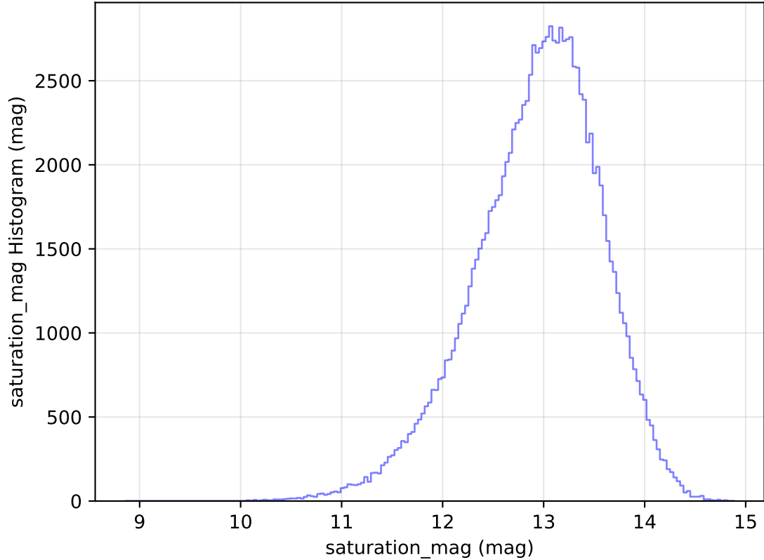
too_elab_heavy_r32_d2_gz_v3.4_10yrs All sky u band: saturation_mag Histogram
