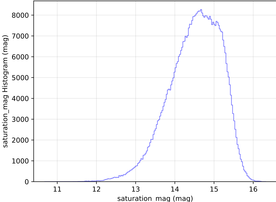
too_elab_heavy_r32_d2_gz_v3.4_10yrs All sky r band: saturation_mag Histogram
