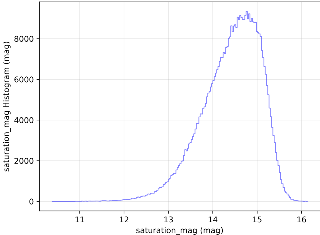
too_elab_heavy_r32_d2_gz_v3.4_10yrs All sky i band: saturation_mag Histogram
