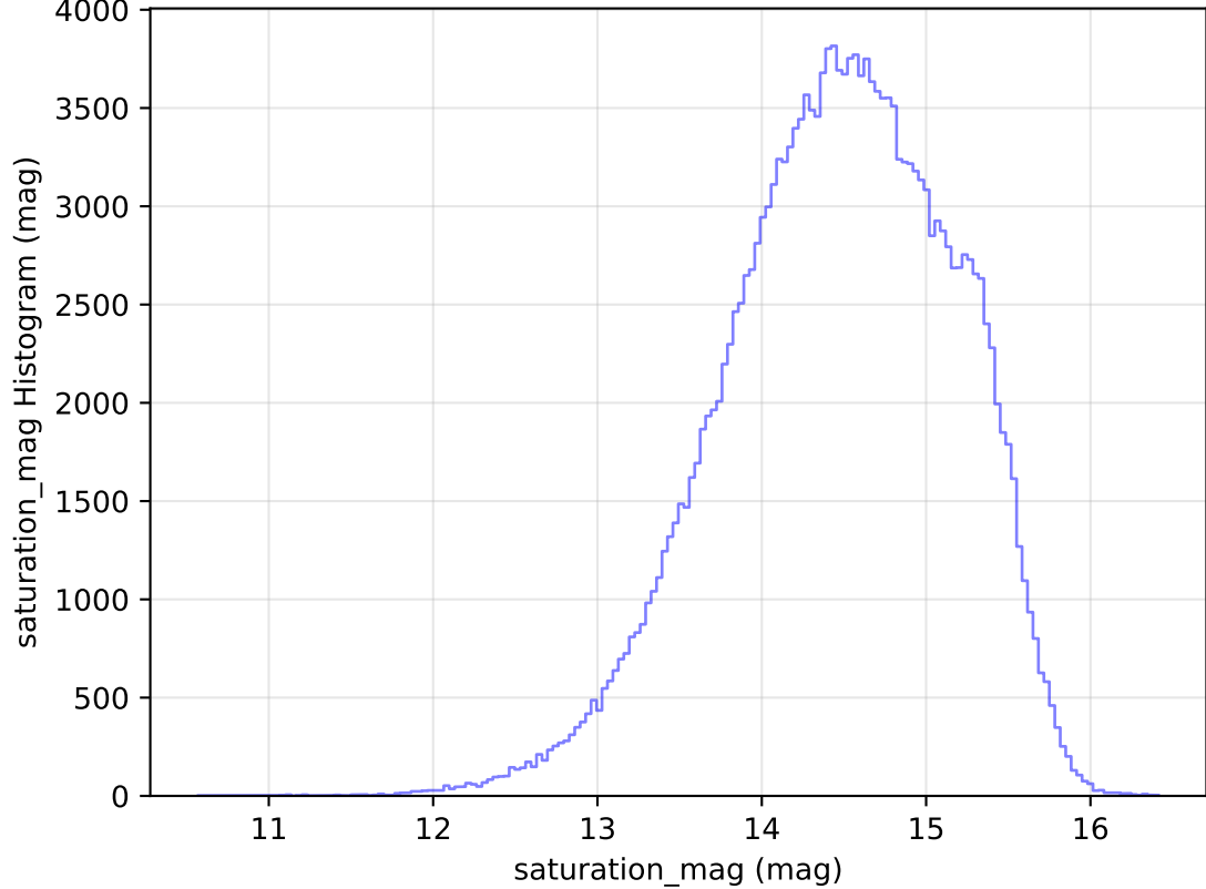
too_elab_heavy_r32_d2_gz_v3.4_10yrs All sky g band: saturation_mag Histogram
