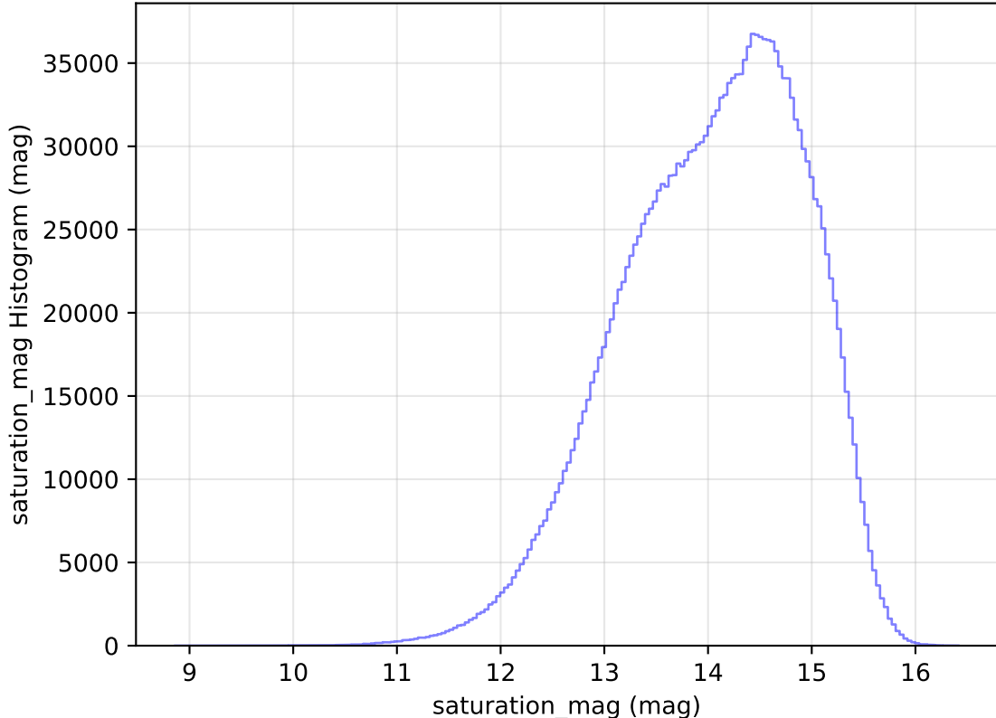
too_elab_heavy_r32_d2_gz_v3.4_10yrs All sky all bands: saturation_mag Histogram
