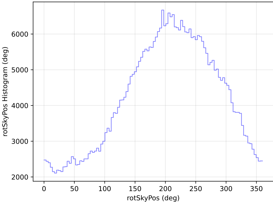
too_elab_heavy_r32_d2_gz_v3.4_10yrs WFD z band: rotSkyPos Histogram
