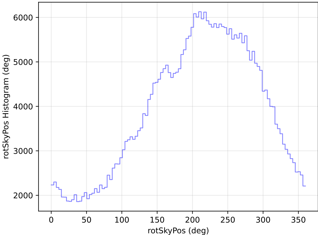
too_elab_heavy_r32_d2_gz_v3.4_10yrs WFD y band: rotSkyPos Histogram
