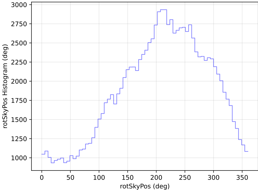
too_elab_heavy_r32_d2_gz_v3.4_10yrs WFD u band: rotSkyPos Histogram
