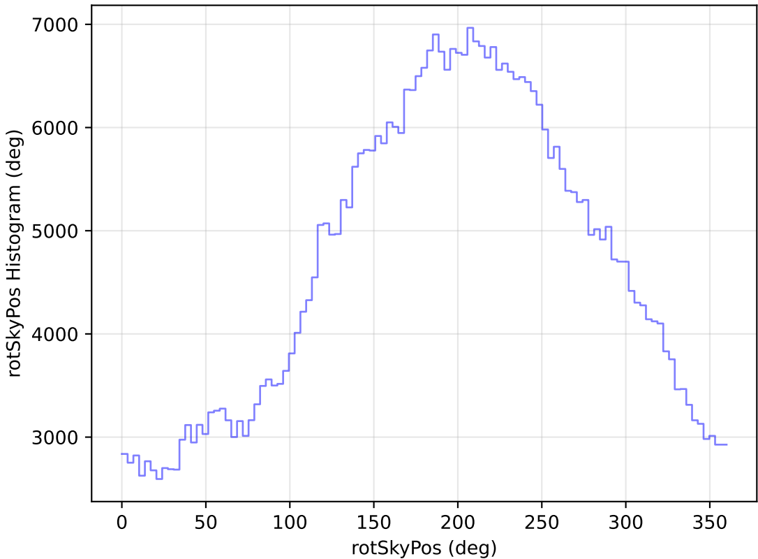
too_elab_heavy_r32_d2_gz_v3.4_10yrs WFD r band: rotSkyPos Histogram
