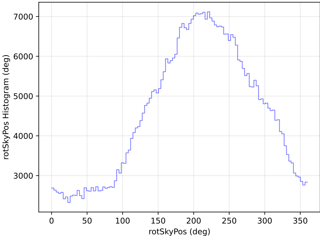
too_elab_heavy_r32_d2_gz_v3.4_10yrs WFD i band: rotSkyPos Histogram
