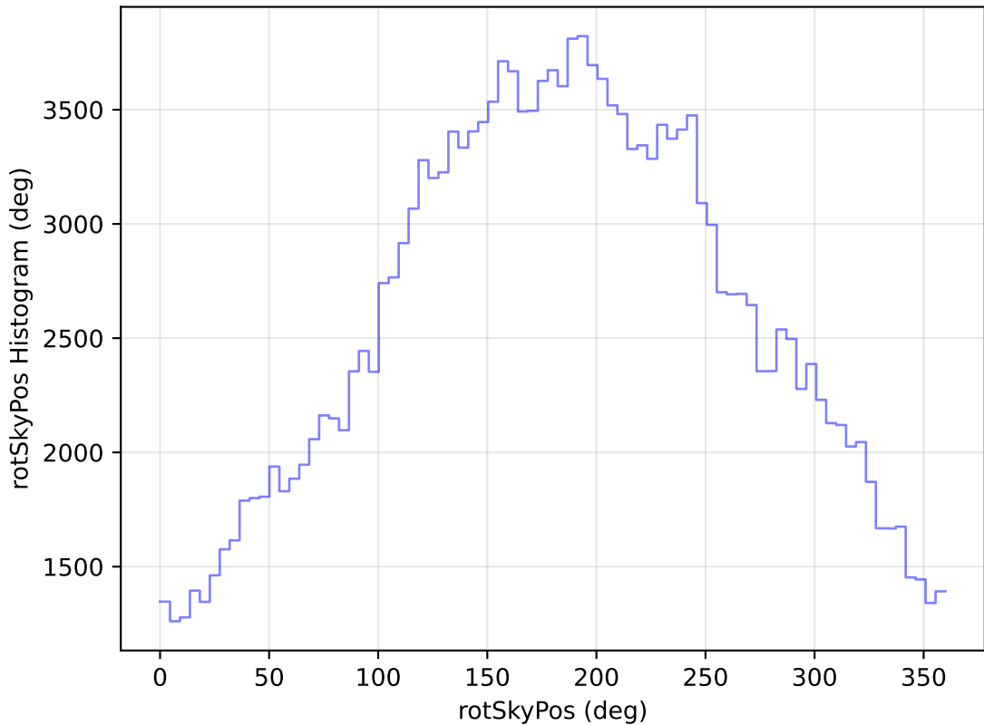
too_elab_heavy_r32_d2_gz_v3.4_10yrs WFD g band: rotSkyPos Histogram
