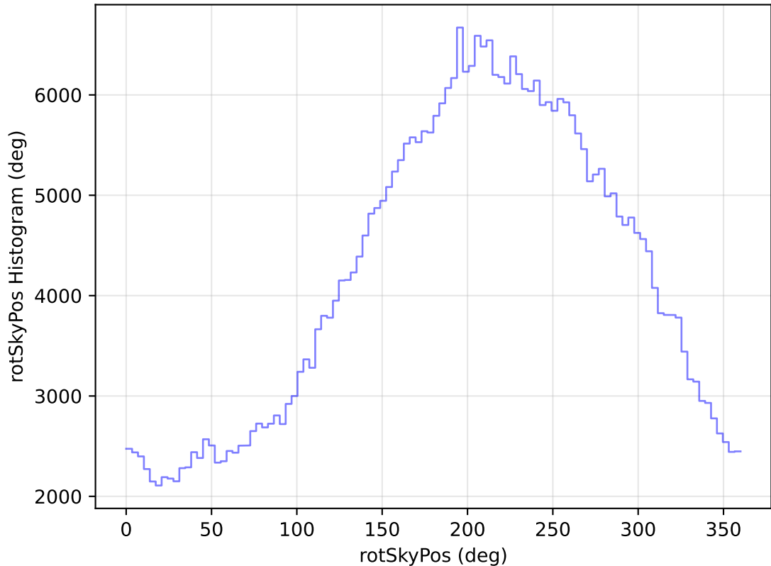
too_elab_heavy_r32_d2_gz_v3.4_10yrs All sky z band: rotSkyPos Histogram
