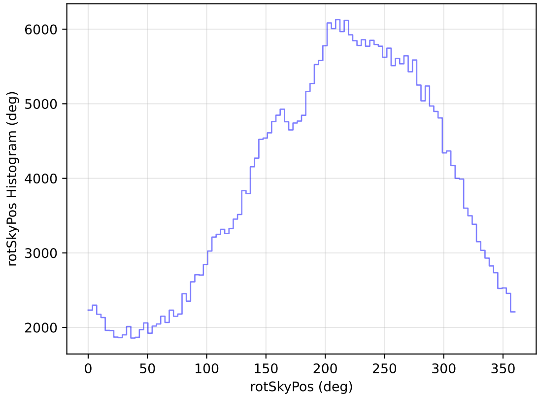
too_elab_heavy_r32_d2_gz_v3.4_10yrs All sky y band: rotSkyPos Histogram
