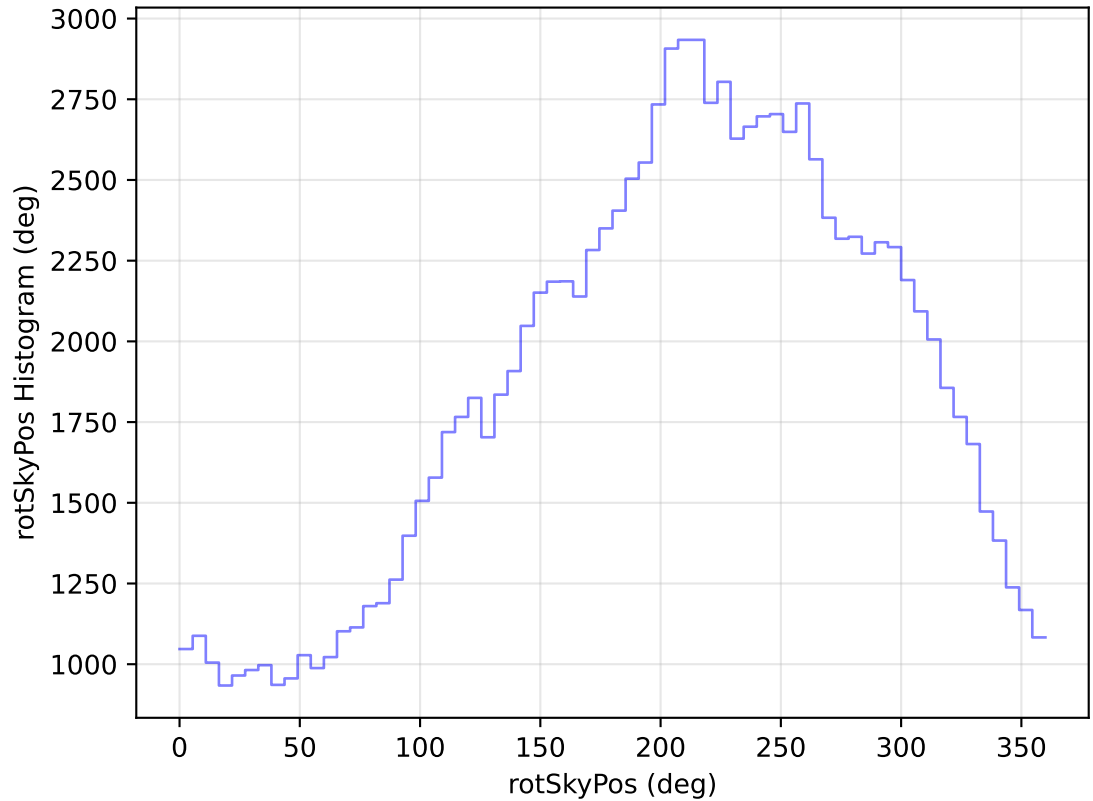
too_elab_heavy_r32_d2_gz_v3.4_10yrs All sky u band: rotSkyPos Histogram
