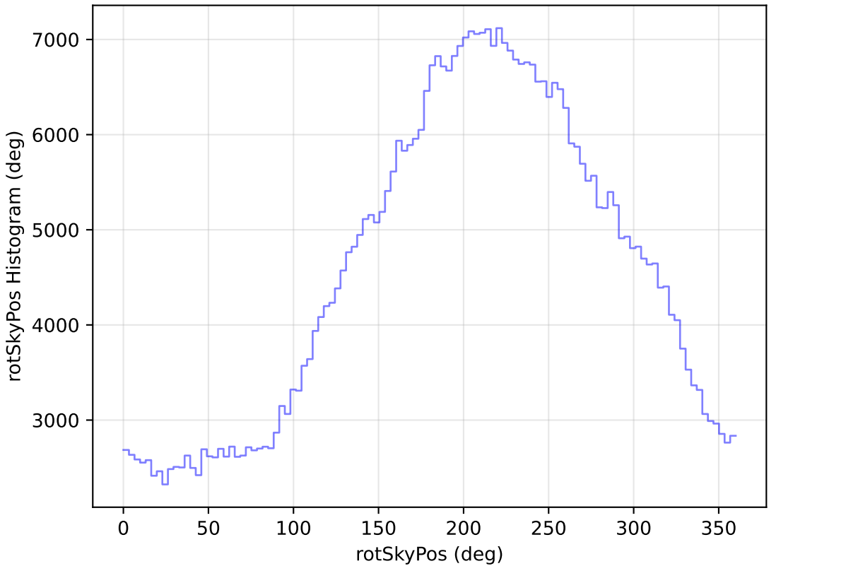
too_elab_heavy_r32_d2_gz_v3.4_10yrs All sky i band: rotSkyPos Histogram
