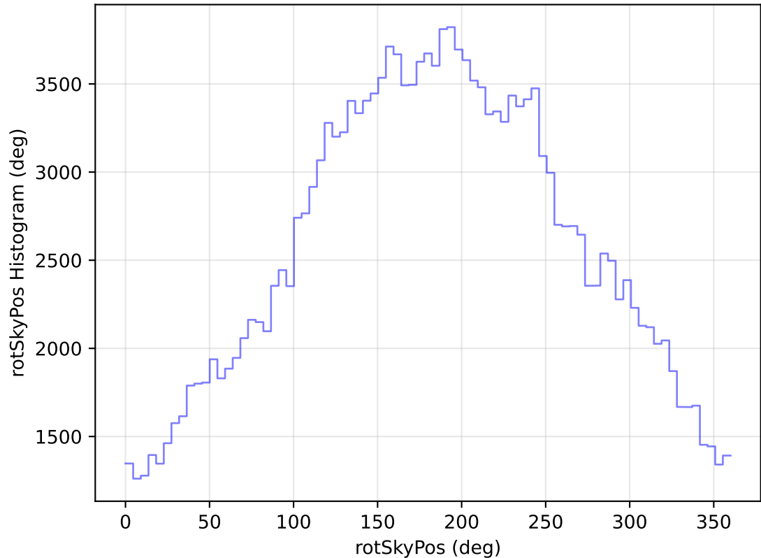
too_elab_heavy_r32_d2_gz_v3.4_10yrs All sky g band: rotSkyPos Histogram
