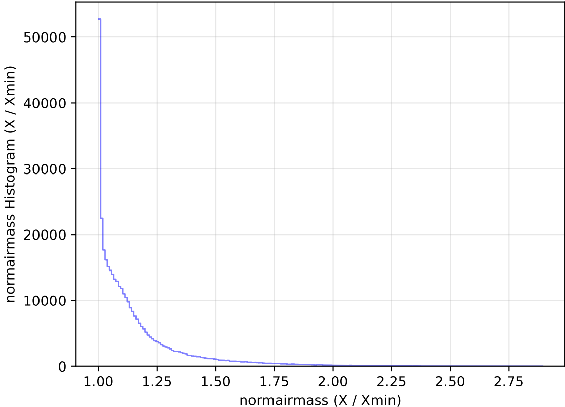
too_elab_heavy_r32_d2_gz_v3.4_10yrs WFD y band: normairmass Histogram
