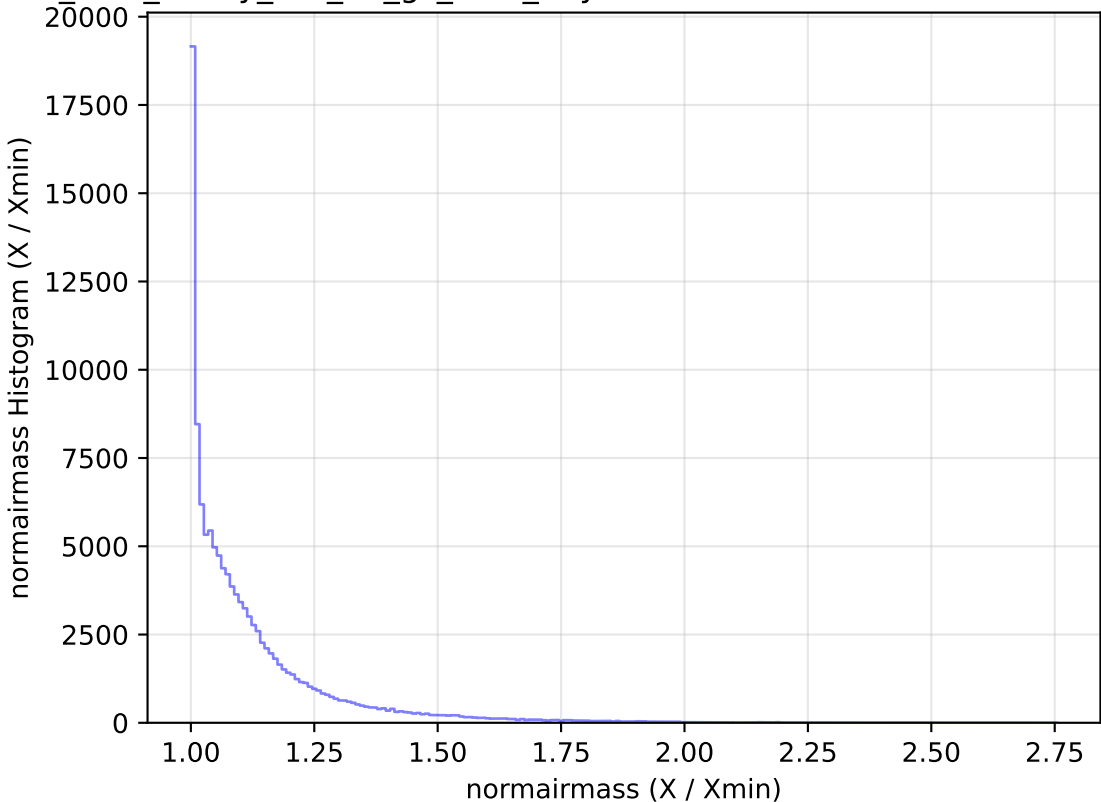
too_elab_heavy_r32_d2_gz_v3.4_10yrs WFD u band: normairmass Histogram
