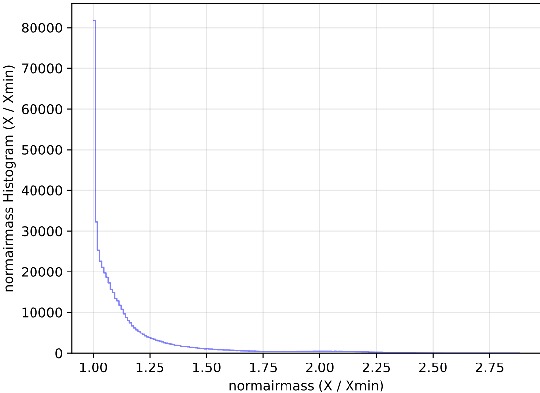
too_elab_heavy_r32_d2_gz_v3.4_10yrs WFD r band: normairmass Histogram
