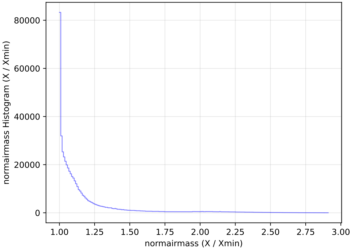
too_elab_heavy_r32_d2_gz_v3.4_10yrs WFD i band: normairmass Histogram
