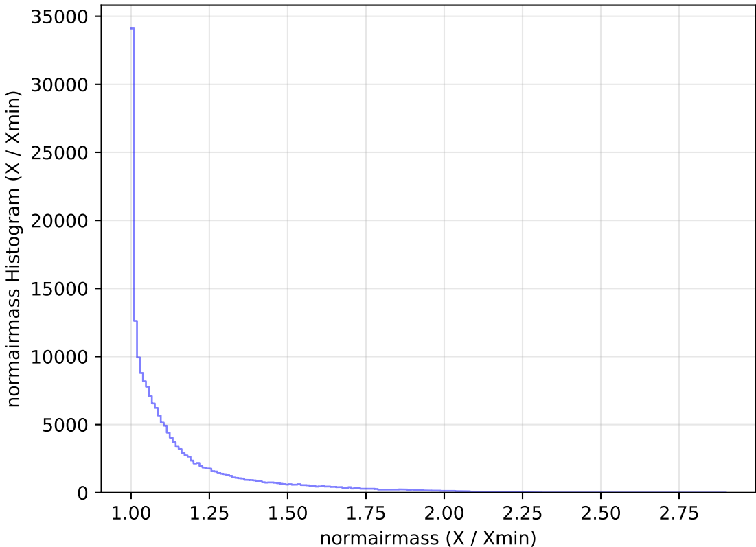
too_elab_heavy_r32_d2_gz_v3.4_10yrs WFD g band: normairmass Histogram
