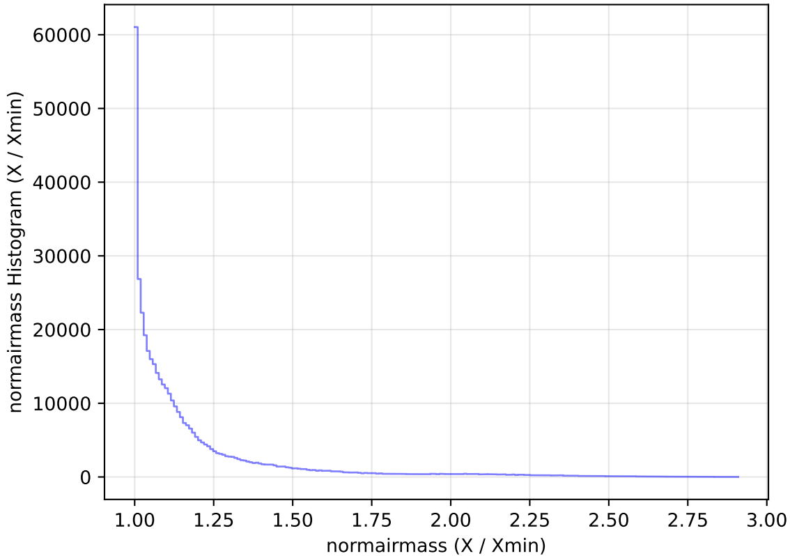
too_elab_heavy_r32_d2_gz_v3.4_10yrs All sky z band: normairmass Histogram
