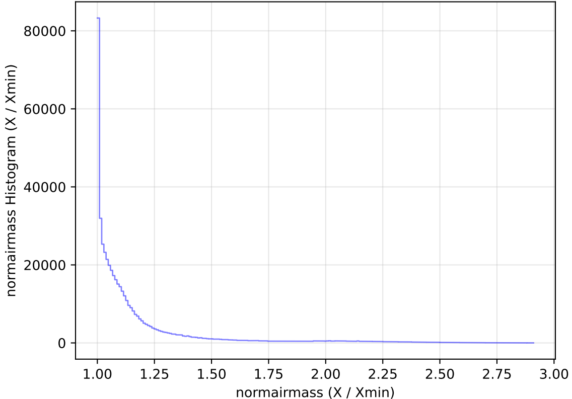
too_elab_heavy_r32_d2_gz_v3.4_10yrs All sky i band: normairmass Histogram
