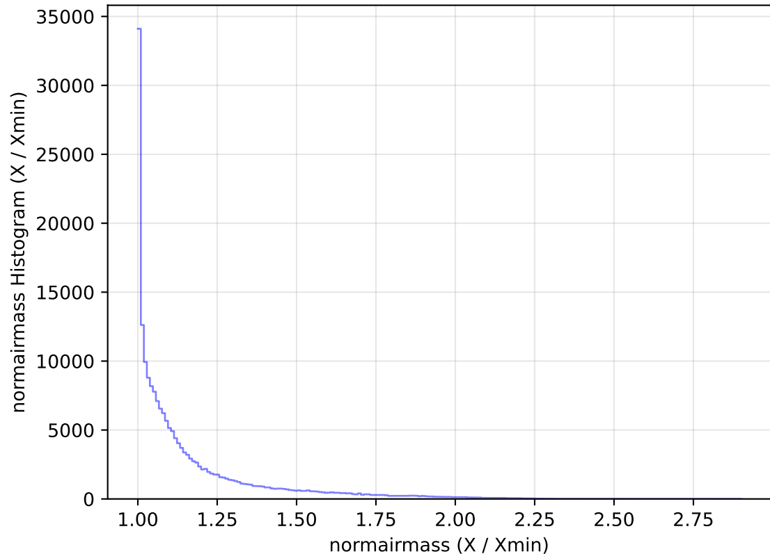
too_elab_heavy_r32_d2_gz_v3.4_10yrs All sky g band: normairmass Histogram
