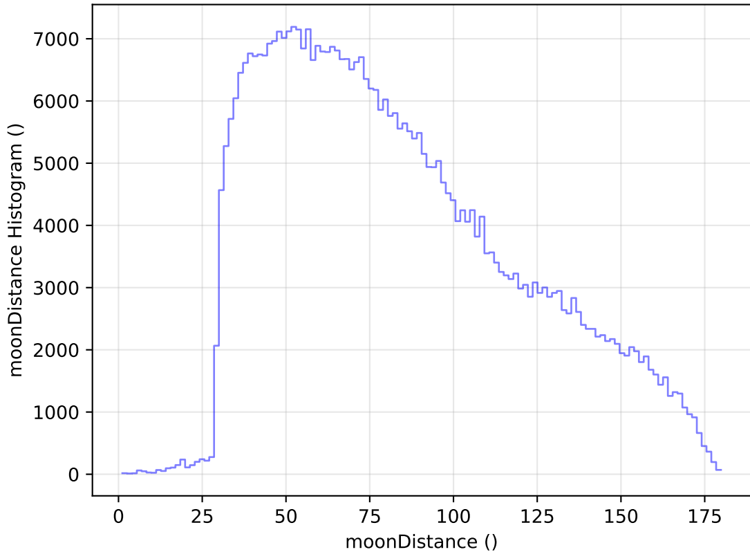
too_elab_heavy_r32_d2_gz_v3.4_10yrs WFD z band: moonDistance Histogram
