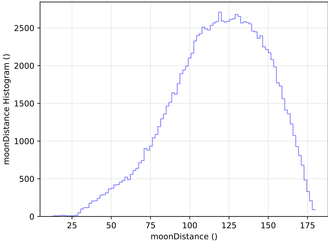
too_elab_heavy_r32_d2_gz_v3.4_10yrs WFD u band: moonDistance Histogram
