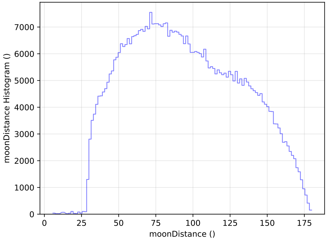
too_elab_heavy_r32_d2_gz_v3.4_10yrs WFD i band: moonDistance Histogram
