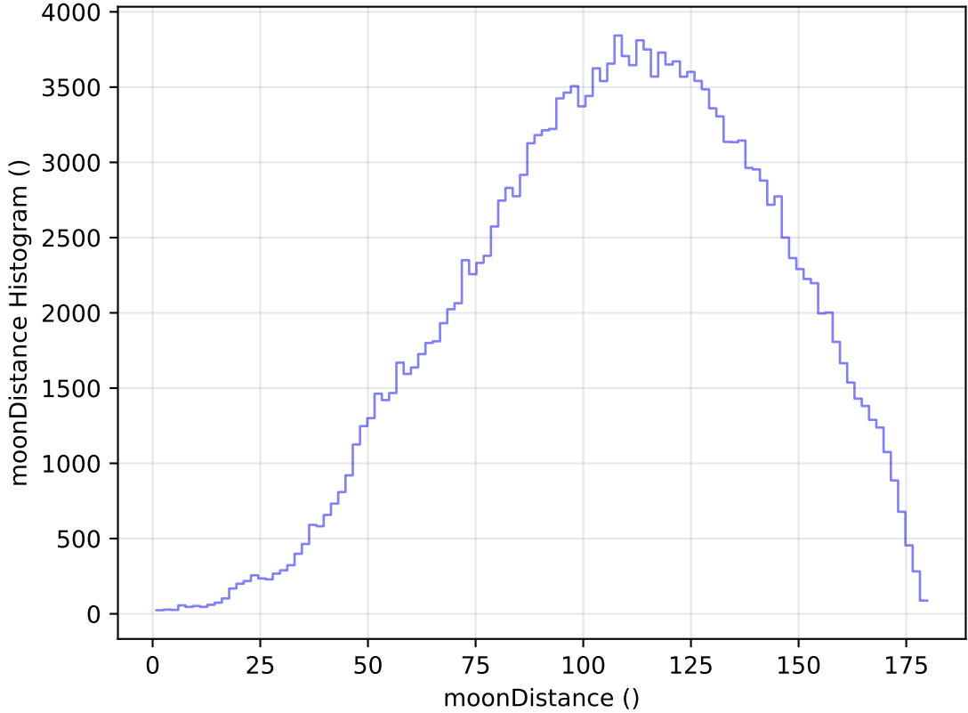
too_elab_heavy_r32_d2_gz_v3.4_10yrs WFD g band: moonDistance Histogram
