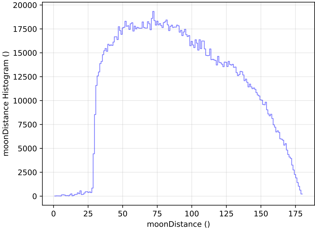
too_elab_heavy_r32_d2_gz_v3.4_10yrs WFD all bands: moonDistance Histogram
