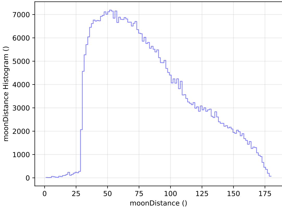
too_elab_heavy_r32_d2_gz_v3.4_10yrs All sky z band: moonDistance Histogram
