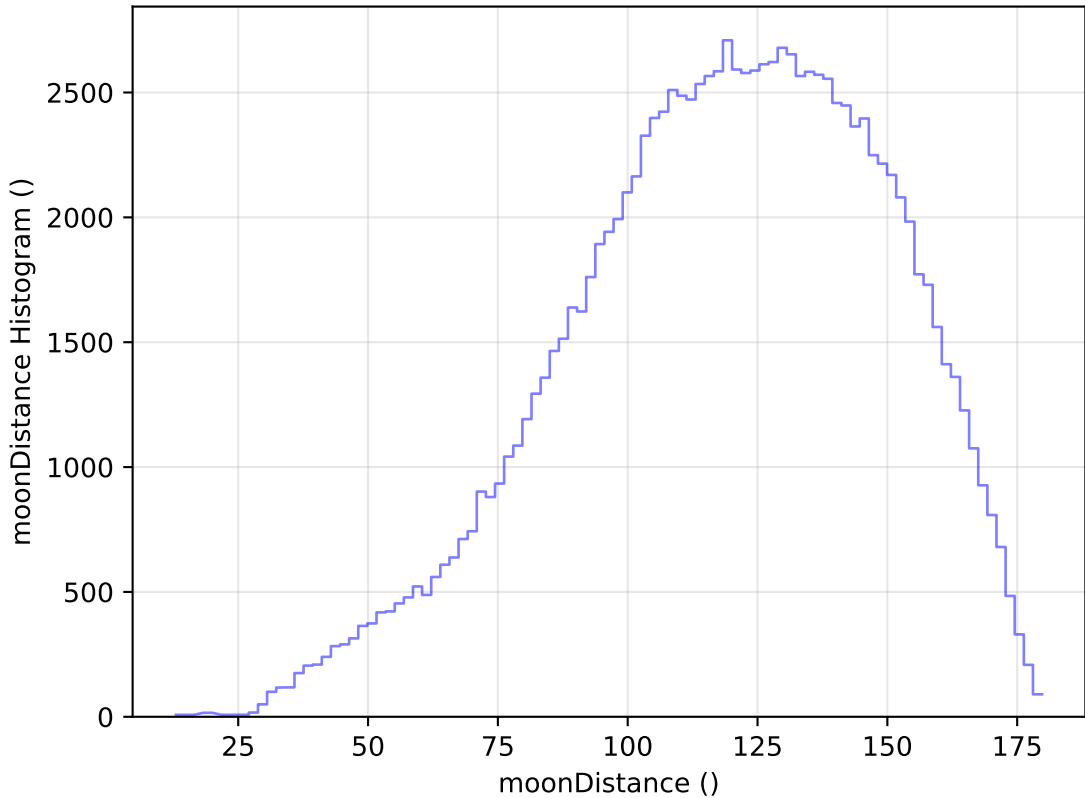
too_elab_heavy_r32_d2_gz_v3.4_10yrs All sky u band: moonDistance Histogram
