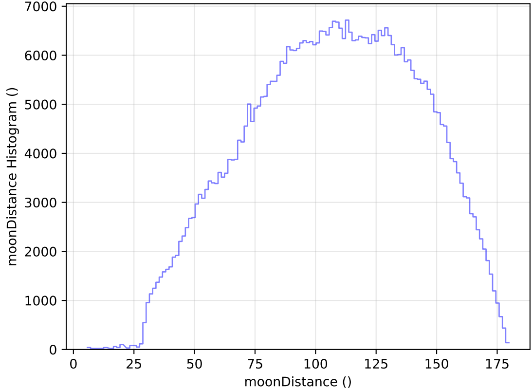
too_elab_heavy_r32_d2_gz_v3.4_10yrs All sky r band: moonDistance Histogram
