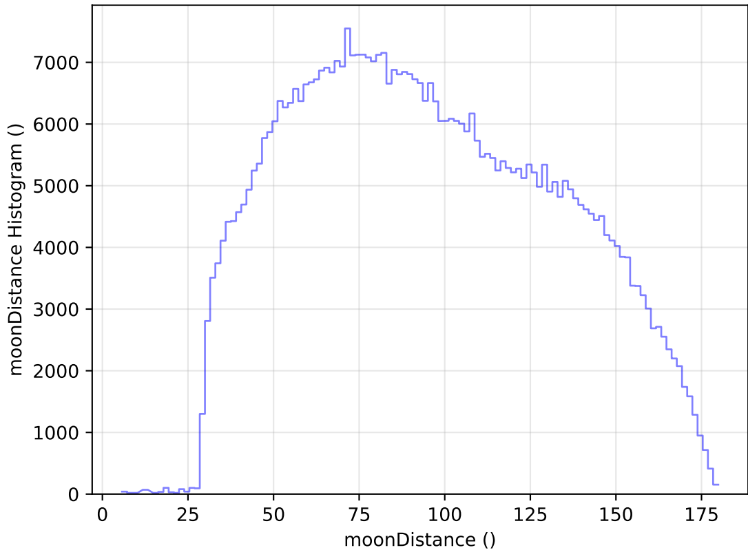
too_elab_heavy_r32_d2_gz_v3.4_10yrs All sky i band: moonDistance Histogram
