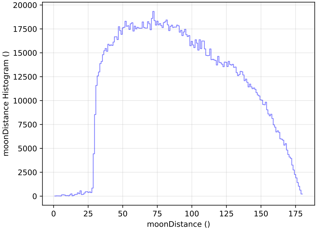
too_elab_heavy_r32_d2_gz_v3.4_10yrs All sky all bands: moonDistance Histogram
