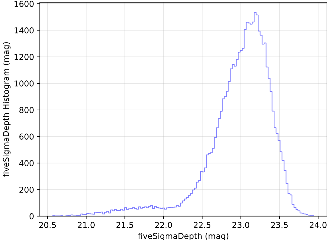
too_elab_heavy_r32_d2_gz_v3.4_10yrs Yr 1 z band: fiveSigmaDepth Histogram
