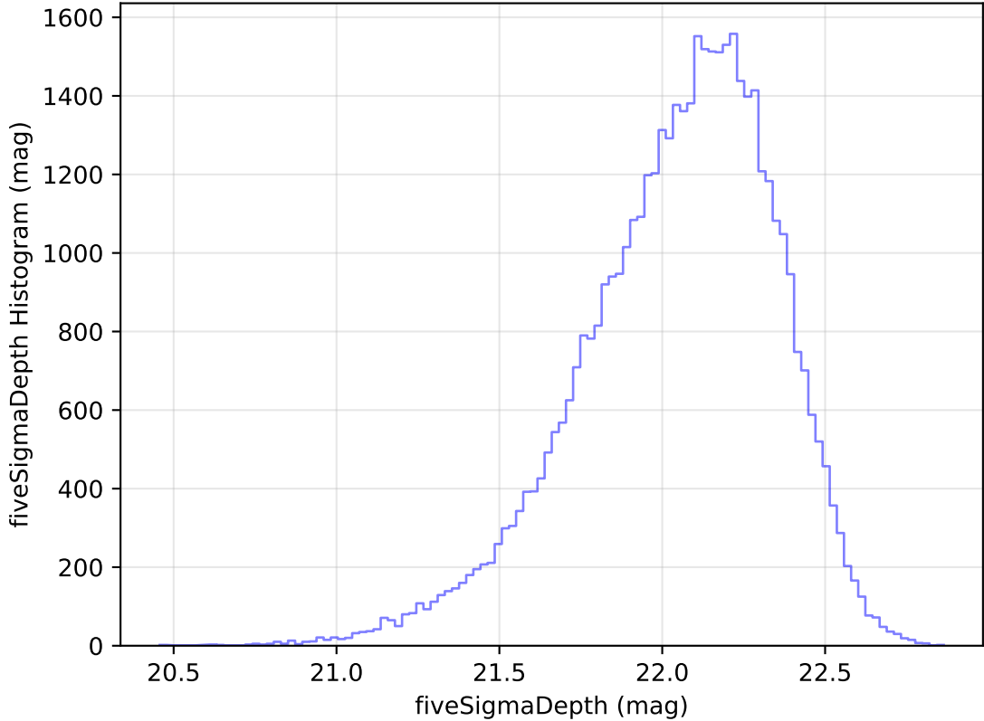
too_elab_heavy_r32_d2_gz_v3.4_10yrs Yr 1 y band: fiveSigmaDepth Histogram
