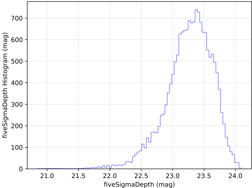
too_elab_heavy_r32_d2_gz_v3.4_10yrs Yr 1 u band: fiveSigmaDepth Histogram
