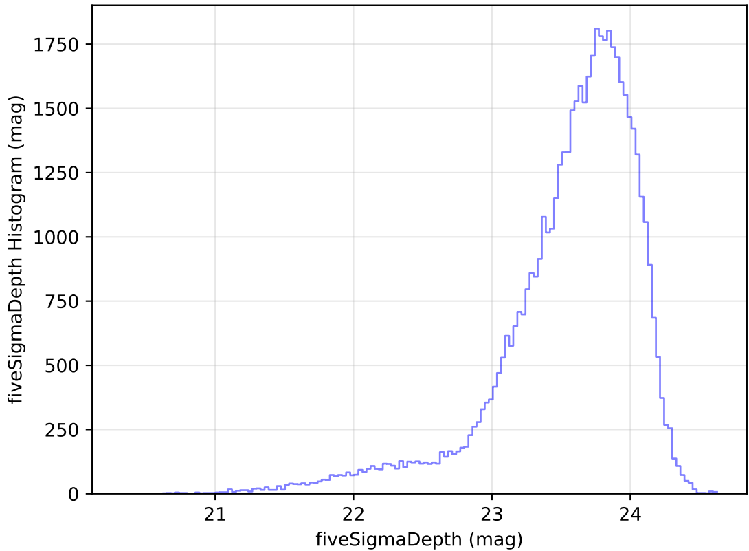
too_elab_heavy_r32_d2_gz_v3.4_10yrs Yr 1 i band: fiveSigmaDepth Histogram
