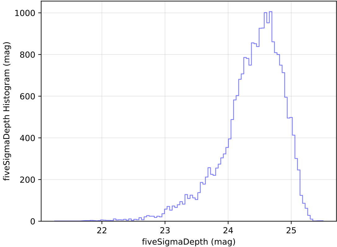
too_elab_heavy_r32_d2_gz_v3.4_10yrs Yr 1 g band: fiveSigmaDepth Histogram
