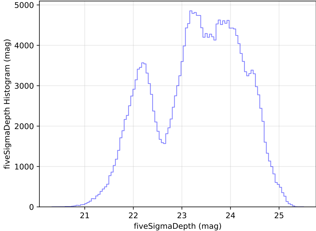
too_elab_heavy_r32_d2_gz_v3.4_10yrs Yr 1 all bands: fiveSigmaDepth Histogram
