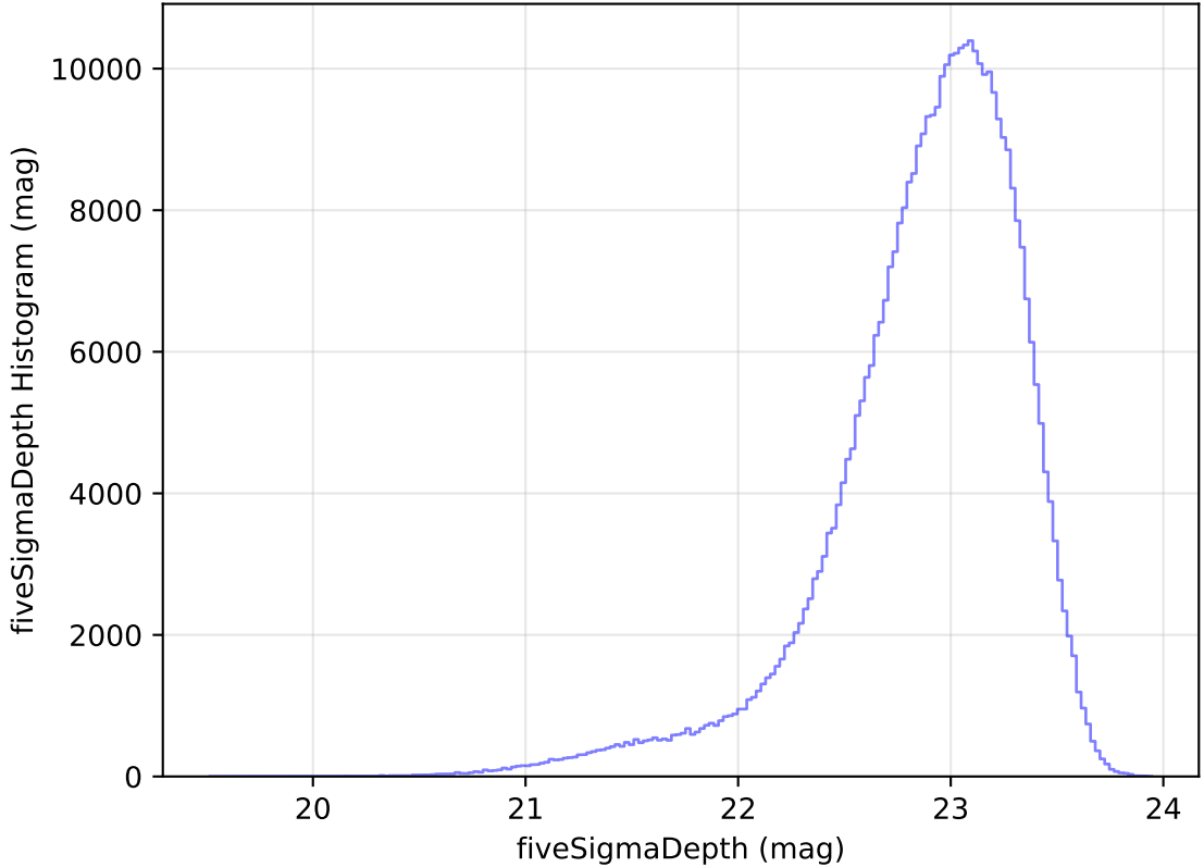
too_elab_heavy_r32_d2_gz_v3.4_10yrs WFD z band: fiveSigmaDepth Histogram
