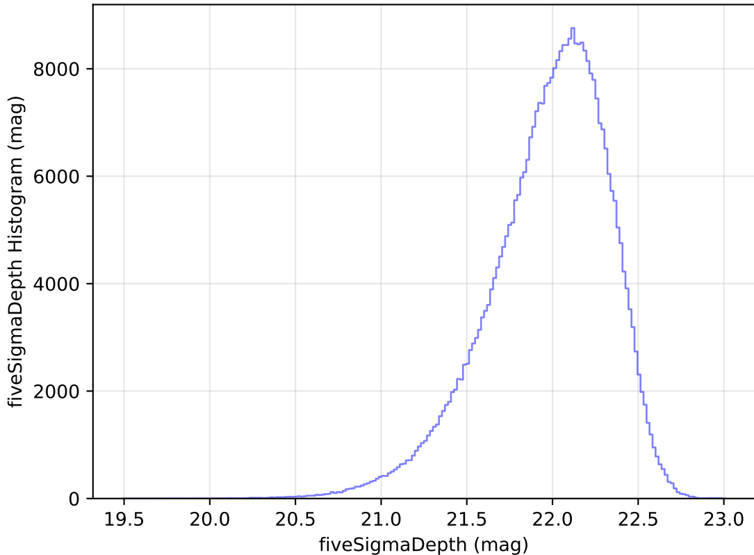
too_elab_heavy_r32_d2_gz_v3.4_10yrs WFD y band: fiveSigmaDepth Histogram
