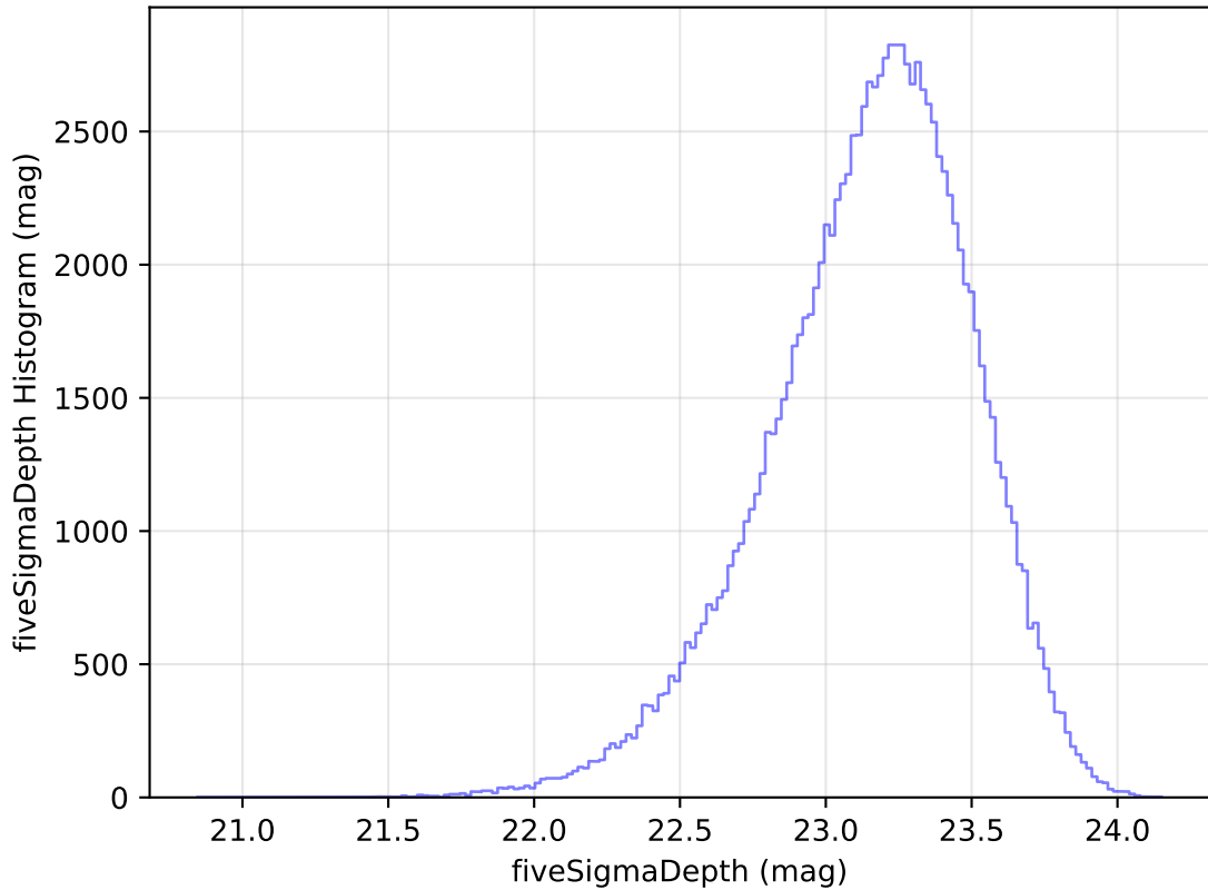
too_elab_heavy_r32_d2_gz_v3.4_10yrs WFD u band: fiveSigmaDepth Histogram
