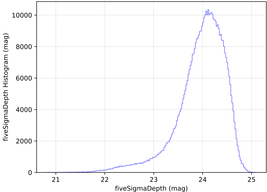
too_elab_heavy_r32_d2_gz_v3.4_10yrs WFD r band: fiveSigmaDepth Histogram
