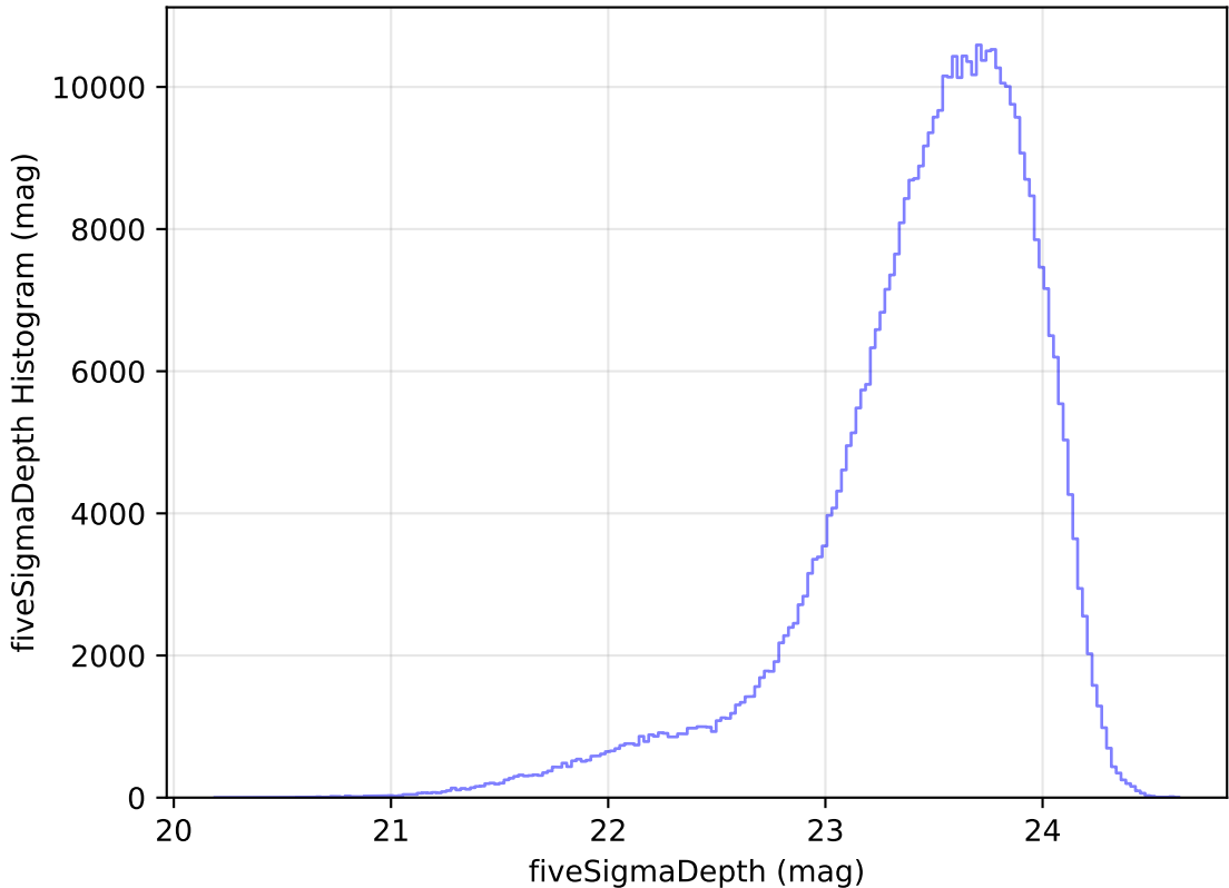
too_elab_heavy_r32_d2_gz_v3.4_10yrs WFD i band: fiveSigmaDepth Histogram
