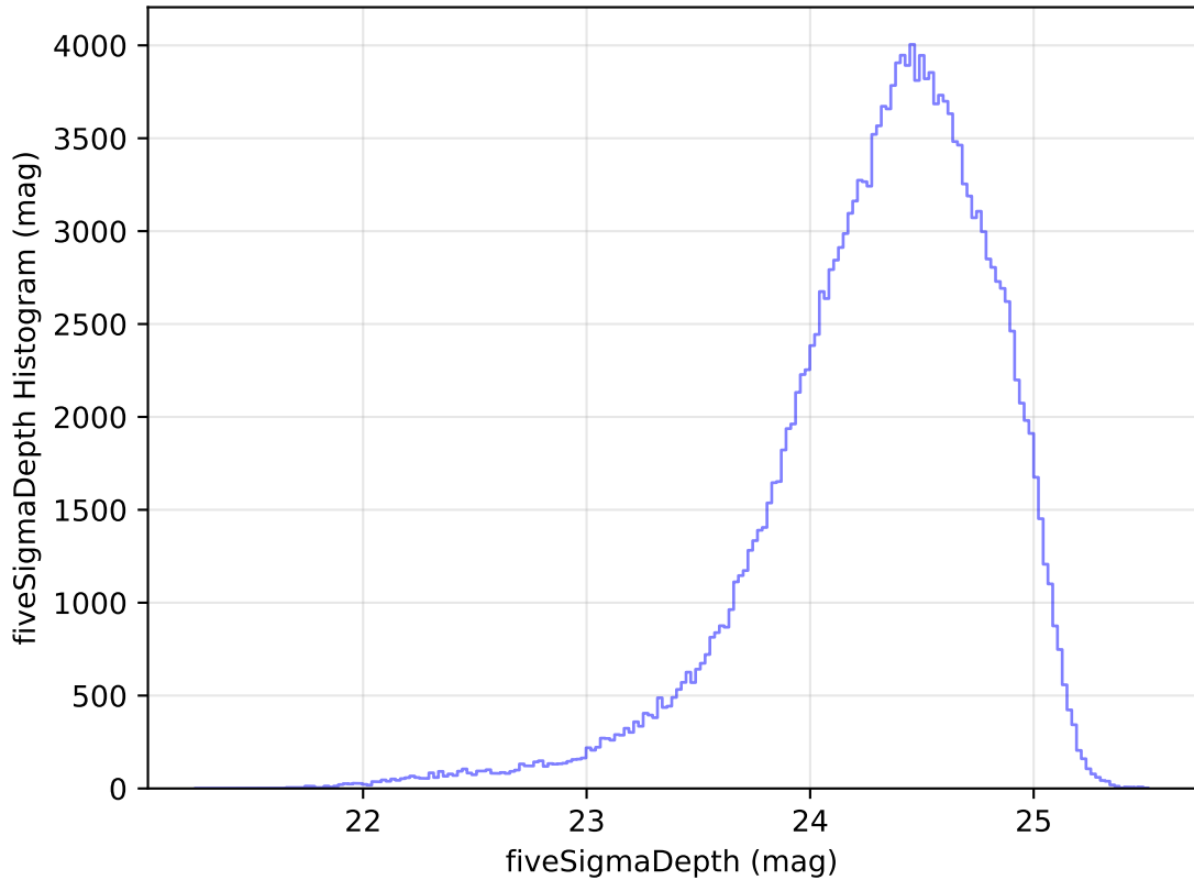
too_elab_heavy_r32_d2_gz_v3.4_10yrs WFD g band: fiveSigmaDepth Histogram
