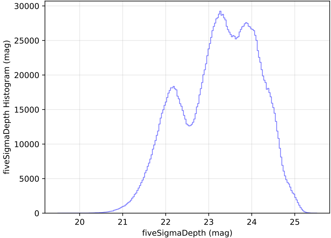
too_elab_heavy_r32_d2_gz_v3.4_10yrs WFD all bands: fiveSigmaDepth Histogram
