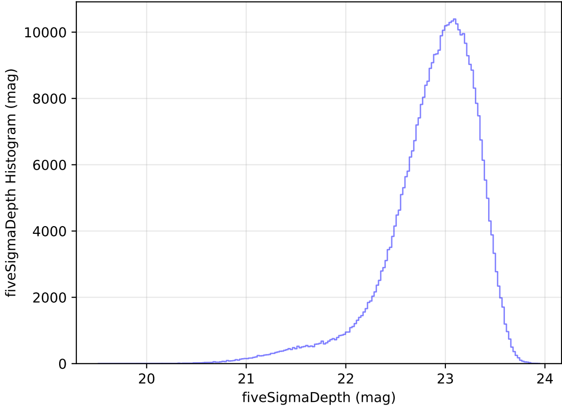
too_elab_heavy_r32_d2_gz_v3.4_10yrs All sky z band: fiveSigmaDepth Histogram
